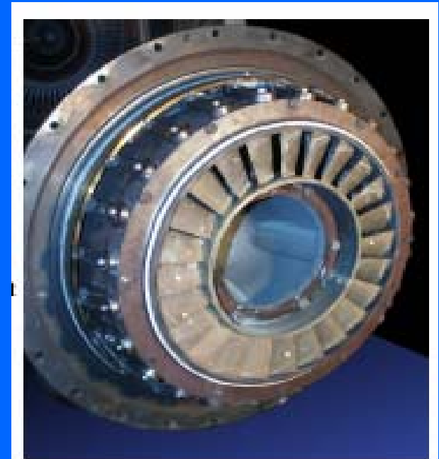
Axial turbine nozzle vanes featuring adjustable throat areas
