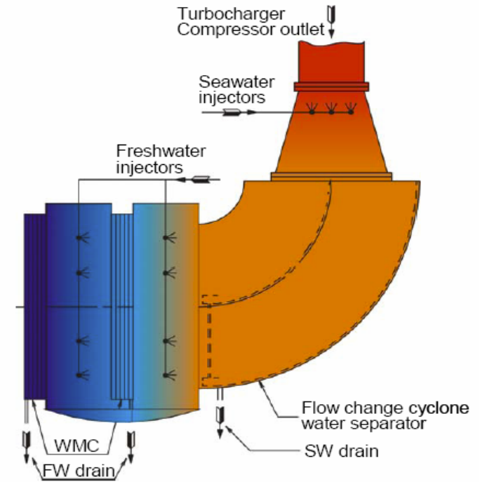
New SAM application versus normal cooler arrangement
