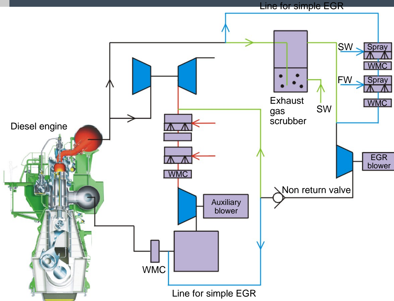
Schematic Design of EGR
