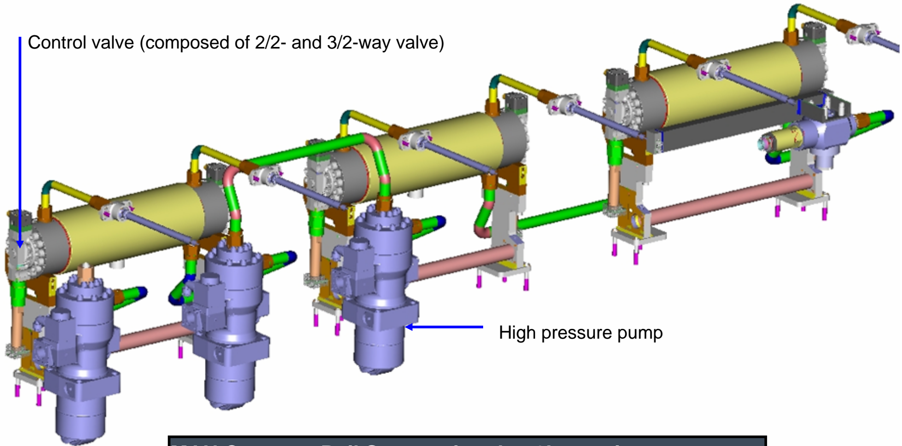
MAN Common Rail System for the 6L - engine
