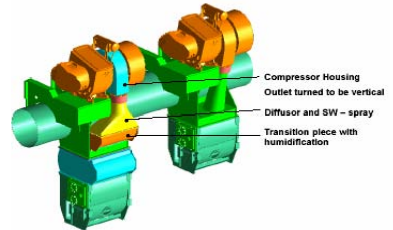
New SAM application versus normal cooler arrangement
