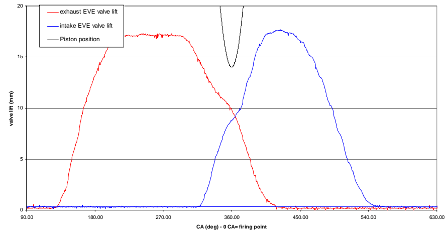
Adjustable valve lift profiles
