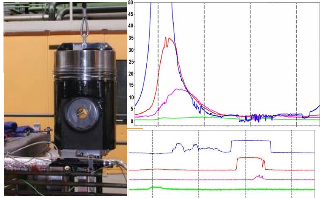
Instrumented Piston
